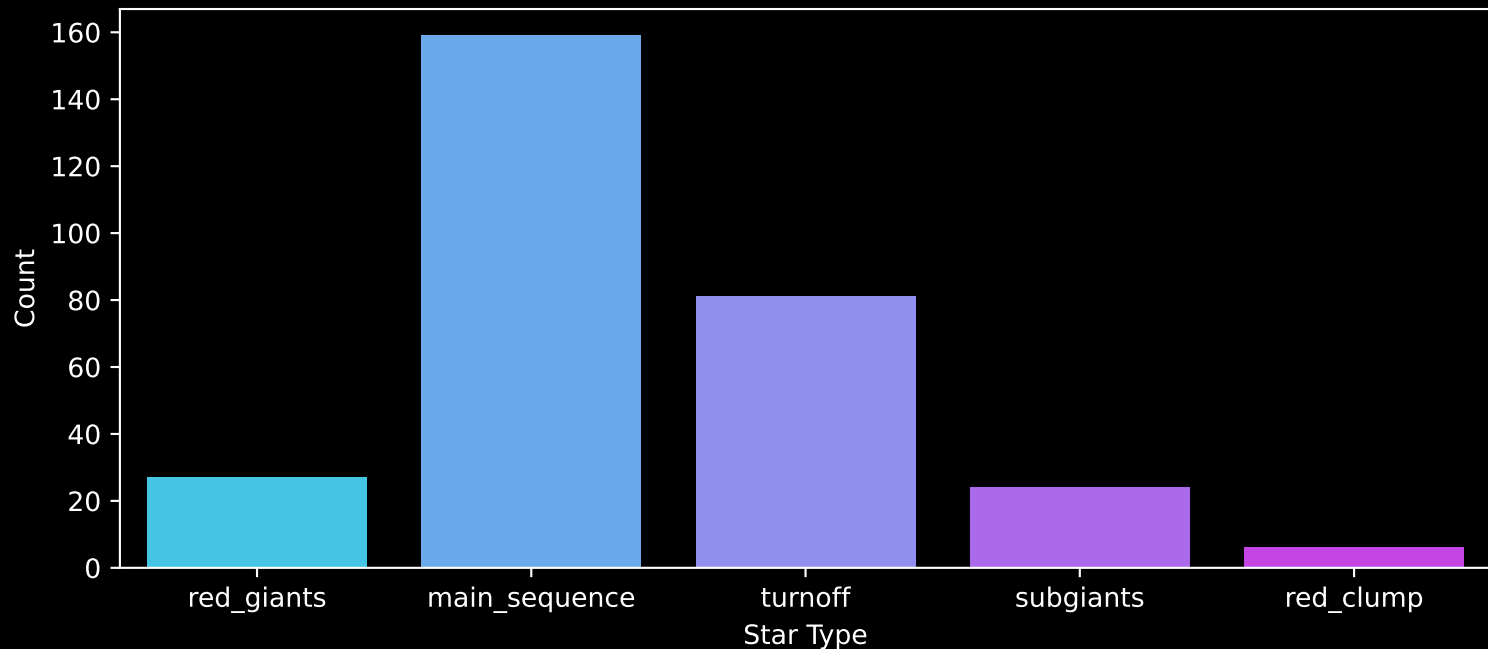
GALAH DR4 Field: [759] Count plot of Star Type
