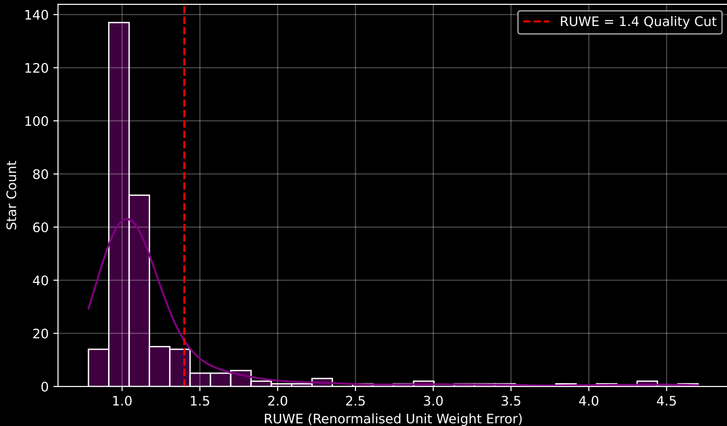
GALAH DR4 Field [759] RUWE Distribution (n= 287)
