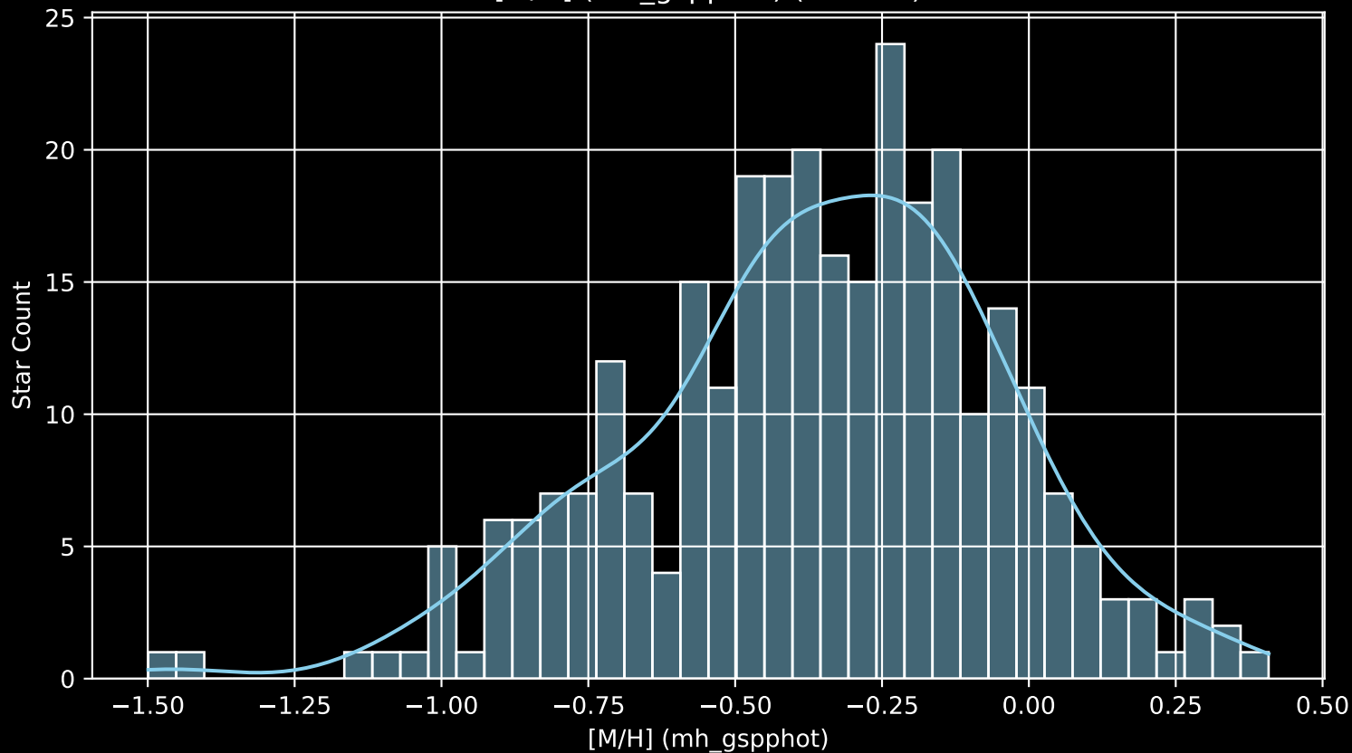
GALAH DR4 Field: [759] [M/H] (mh_gspphot) (n= 297)
